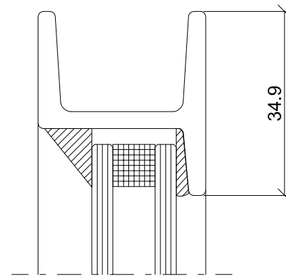
STANDARD FIXED LIGHT WITHOUT TRICKLE VENT.
