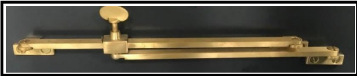
FS1030 Non-locking / FS1034 Locking Double Arm Stay: For side hung casements over 650mm wide. Available for the knurled knob sliding stay too. Additional cost POA.
