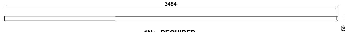
1No. REQUIRED. 50x30x3mm STEEL BOX SECTION.
