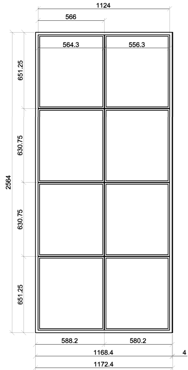
1No. REQUIRED. FIXED LIGHT FRAME.
