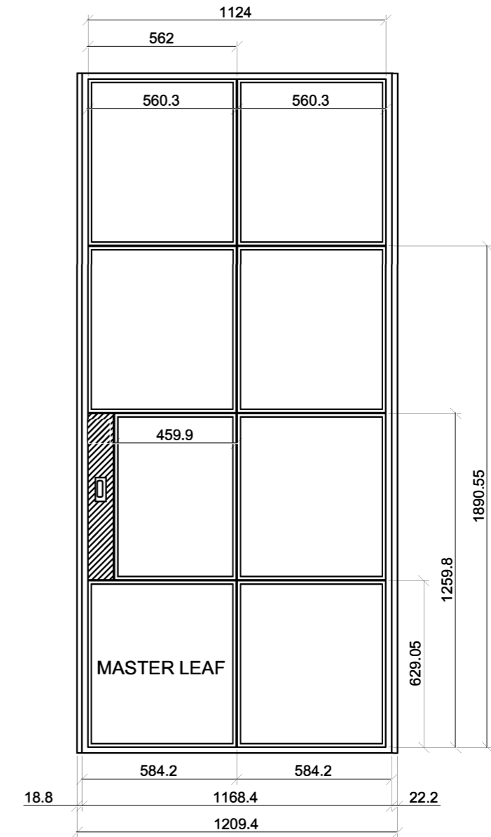
1No. REQUIRED. SLIDING DOOR.
