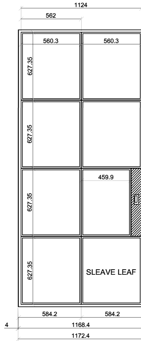
1No. REQUIRED. SLIDING DOOR.
