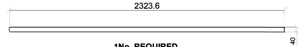
1No. REQUIRED. ALUMINIUM SLIDING TRACK.
