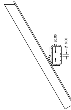
SECTION F-F SCALE 1 / 3
