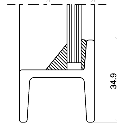
19mm X 19mm TEE BAR SINGLE GLASS ONLY
