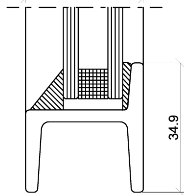
MODIFIED TEE BAR SINGLE OR DOUBLE GLASS
