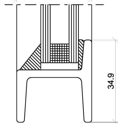
STANDARD TEE BAR SINGLE OR DOUBLE GLASS
